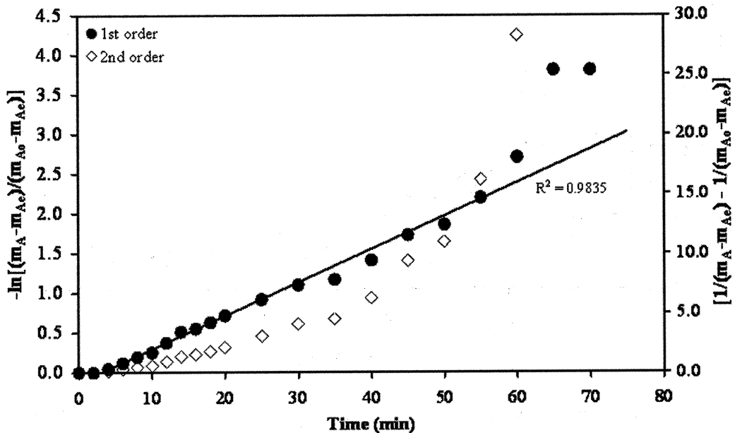
Figure 4. Determination of order of reaction of the combustion of the coal briquette with a moisture content of 10 wt%.
