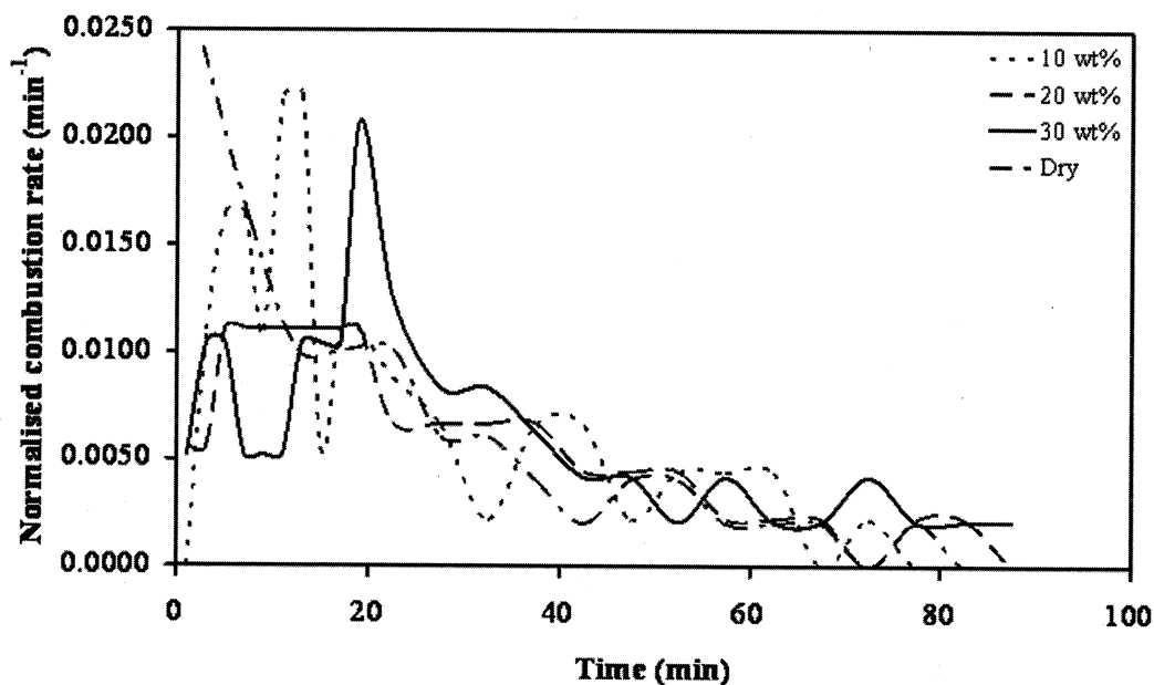
Figure 3. Combustion rates of the coal briquettes with moisture contents of 10-30 wt%, compared with that of the dry coal briquette (from Ref. [9]).
