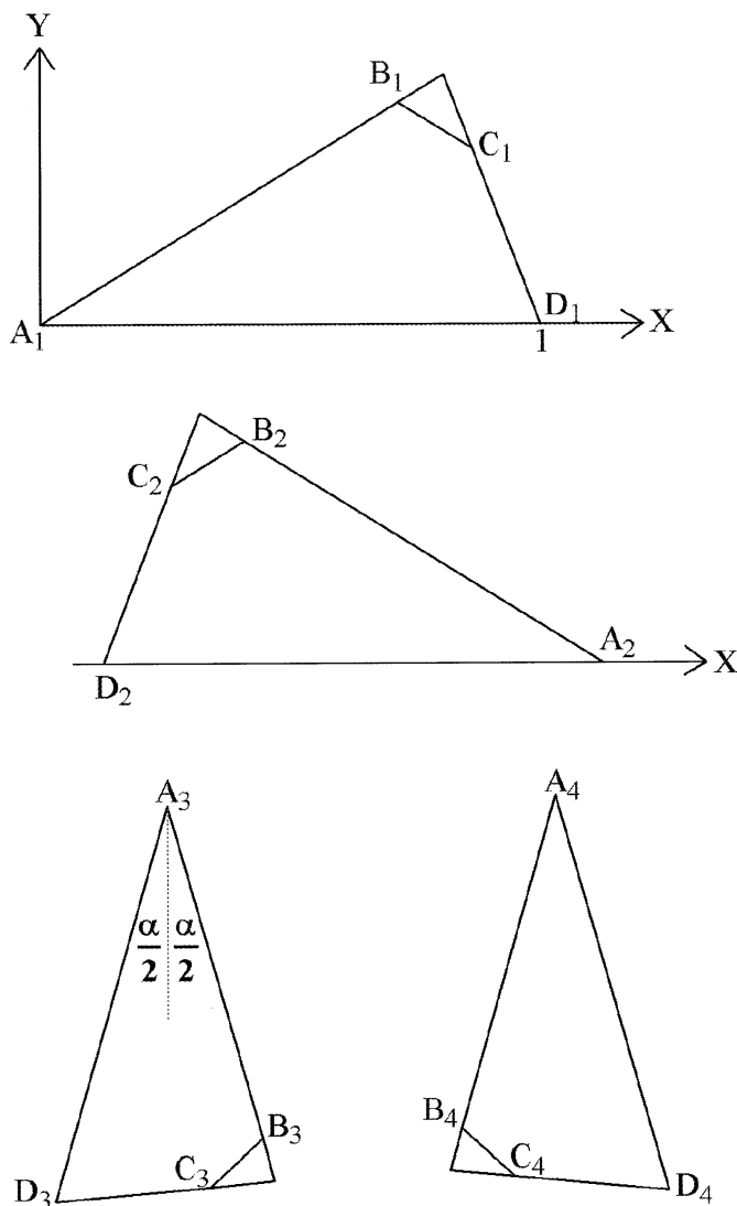
Figure 12. The 4 copies of \bar{T} .
