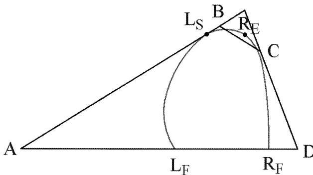
Figure 8. The arc \gamma and \bar{T}_0 .
