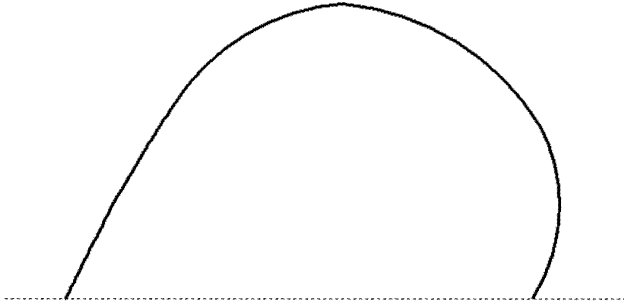
Figure 3. An arc in its “standing post”.
