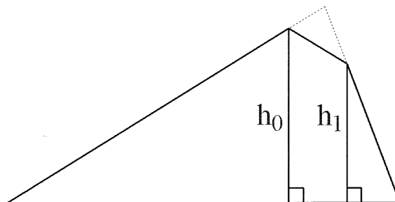
Figure 2. The quadrilateral \bar{T} .
