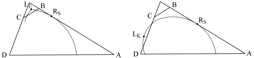
Figure 9. The arc \gamma and \overline{T}^1 .
