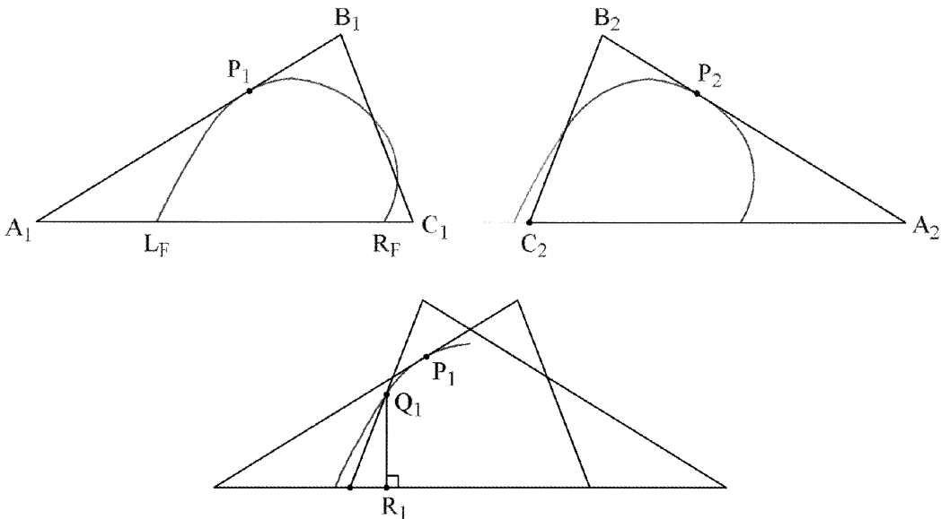
Figure 4. Translation of \gamma into T and T^\perp .
